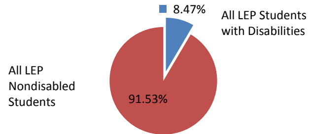
LEP Students with Disabilities (SWD) to All LEP Students
